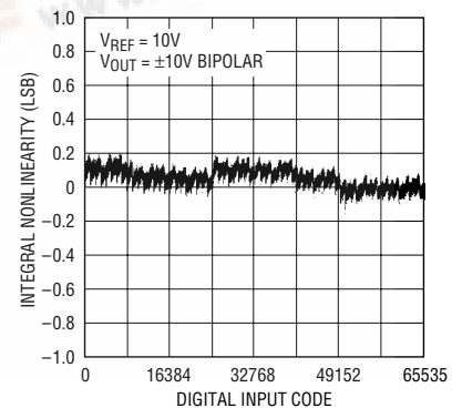
LTC1821/LTC1821-1 Integral Nonlinearity
