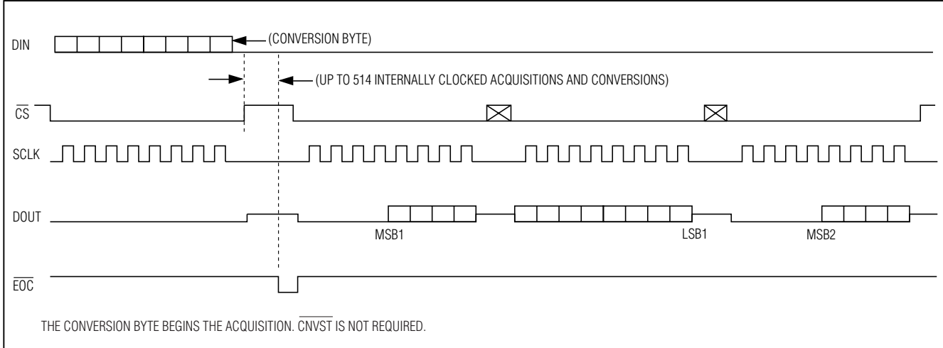
Figure 6. Clock Mode 10
