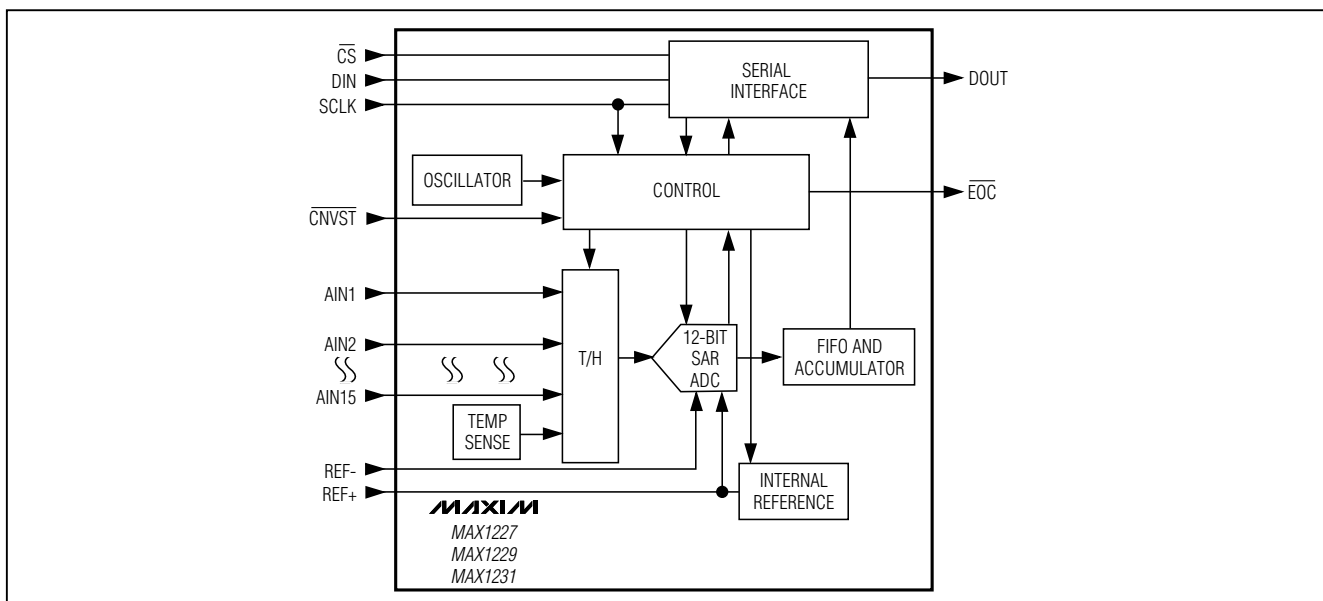
Figure 2. Functional Diagram
