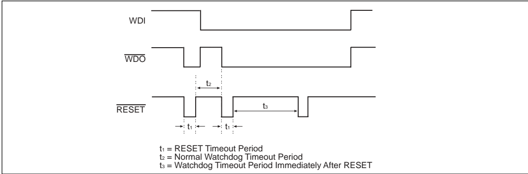
Figure 20. Watchdog Timeout Period and Reset Active Time
