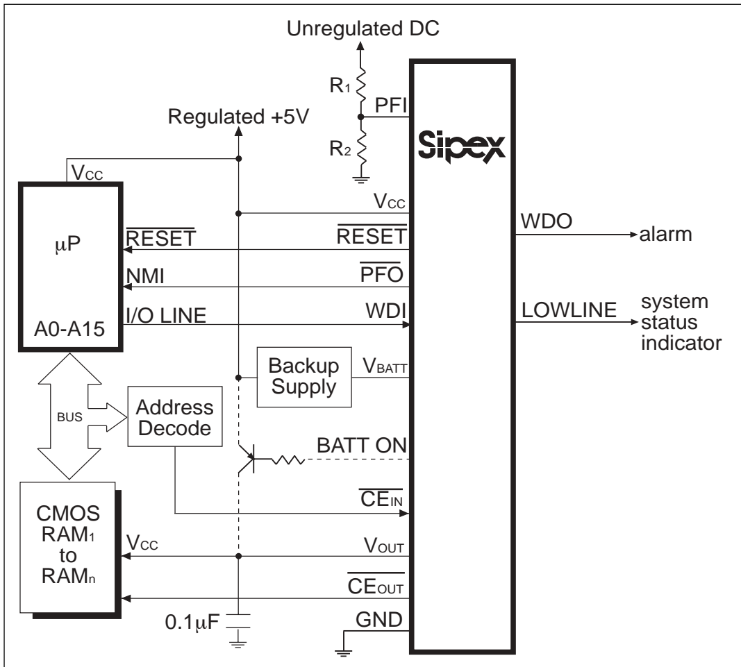
Figure 17. Typical Application Circuit of the SP691A/693A/800L/800M
