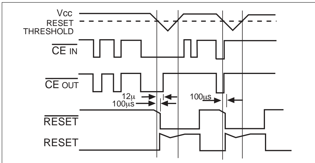
Figure 19. Reset and CE In/Out Timing
