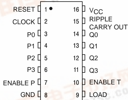
Figure 1. Pin Assignment
