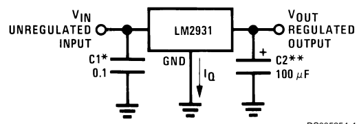
LM2931 Fixed Output
