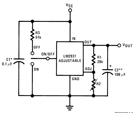
LM2931 Adjustable Output
