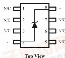
8-Pin Surface Mount (S)
