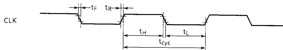
Figure 6.1 System Clock
