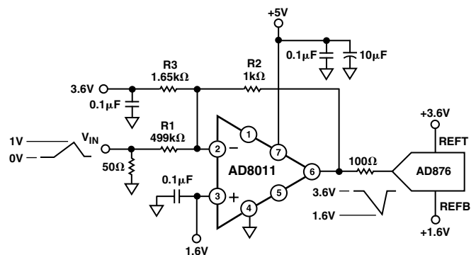
Figure 36. AD8011 Driving the AD876
