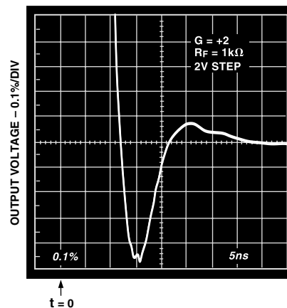
Figure 20. Short-Term Settling Time; V_S = +5\text{ V or } \pm 5\text{ V}
