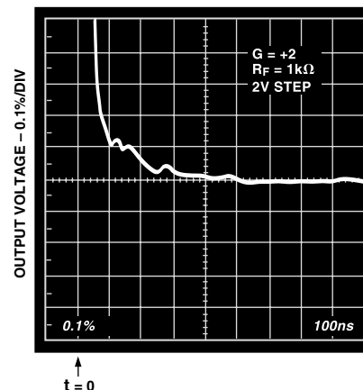
Figure 21. Long-Term Settling Time; V_S = +5\text{ V or } \pm 5\text{ V}
