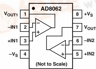
SOIC-8 (R) and \mu SOIC (RM)
