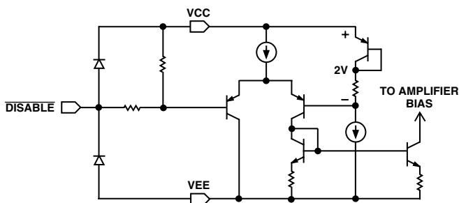
Figure 10. Disable Circuit of the AD8063
