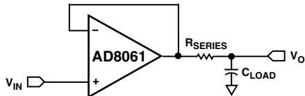
Figure 8. Series Resistor Isolating Capacitive Load
