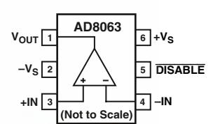
SOT-23-6 (RT)
