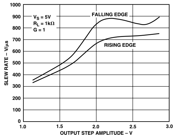
TPC 18. Slew Rate vs. Output Step Amplitude
