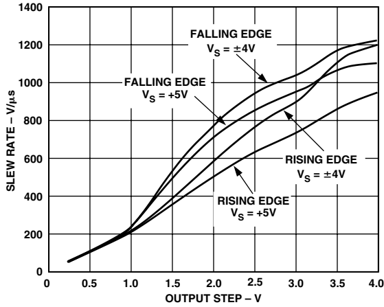
TPC 19. Slew Rate vs. Output Step Amplitude, G = 2 , R_L = 1\text{ k}\Omega , V_S = 5\text{ V}
