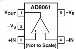
SOT-23-5 (RT)
