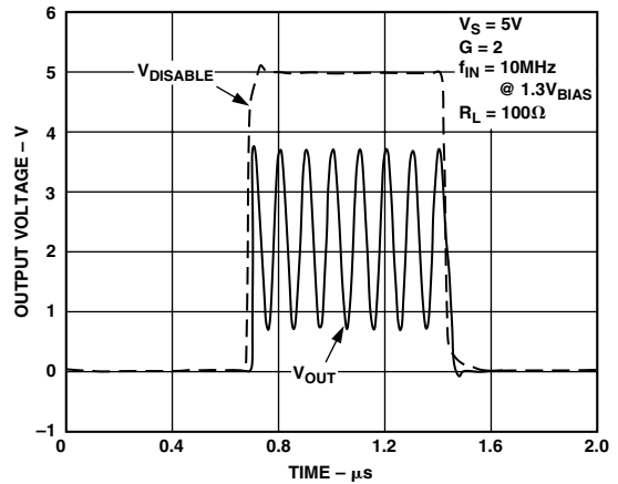
TPC 29. \overline{DISABLE} Function, Voltage = 0 V to 5 V
