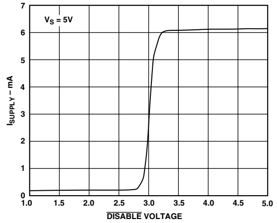
TPC 28. \overline{DISABLE} Voltage vs. Supply Current
