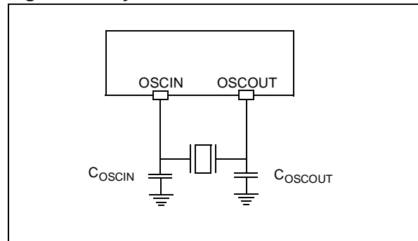
Figure 17. Crystal Resonator
