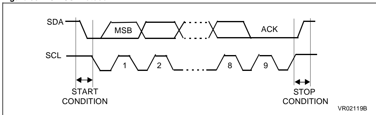
Figure 66. I 2 C BUS Protocol
