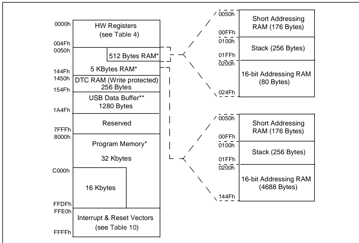
Figure 11. Memory Map
