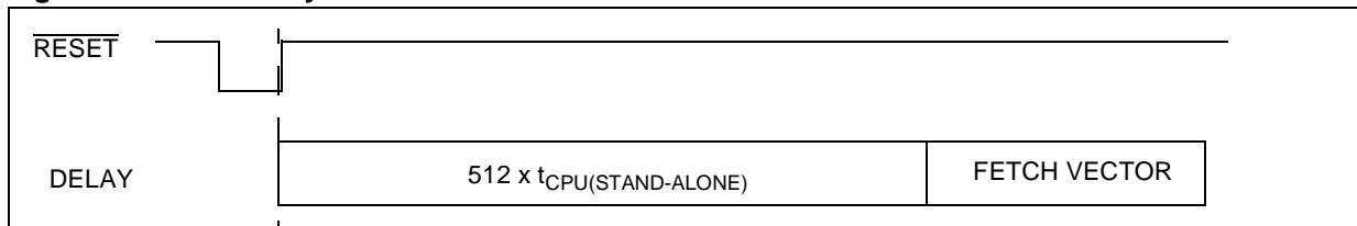
Figure 20. Reset Delay in Stand-alone Mode
