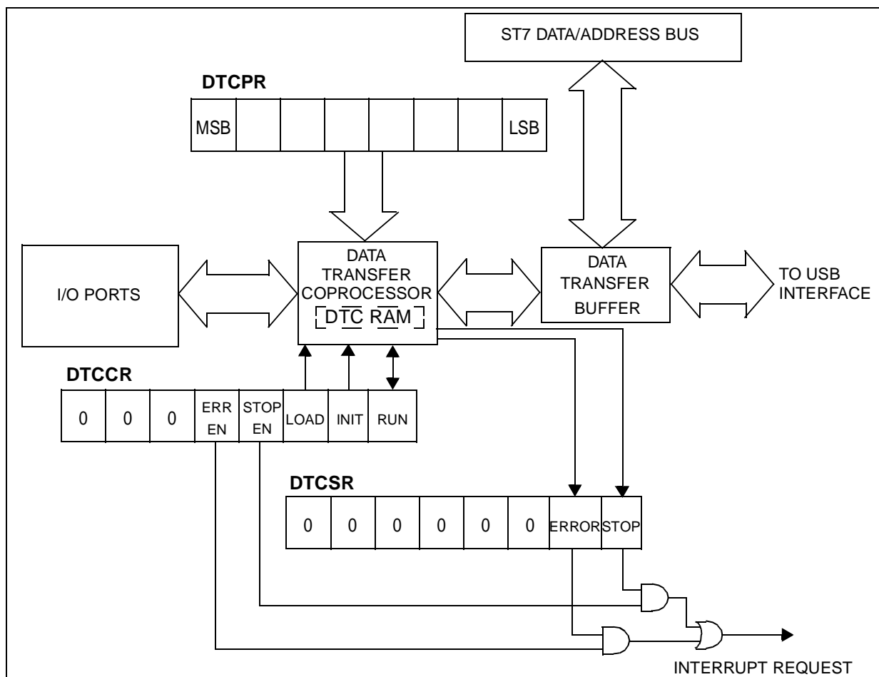
Figure 38. DTC Block Diagram
