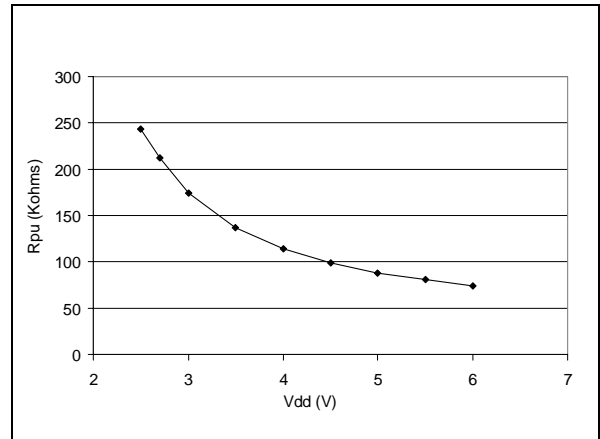
Figure 90. Typical R_{PU} vs. V_{DD} with V_{IN}=V_{SS}
