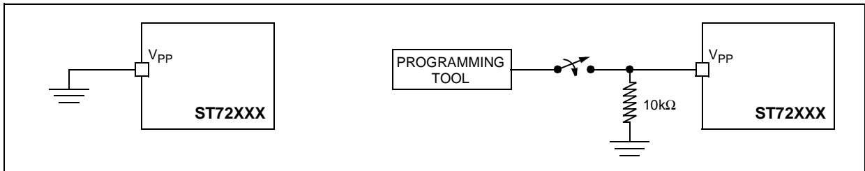
Figure 78. Two typical Applications with V_{PP} Pin 1)
