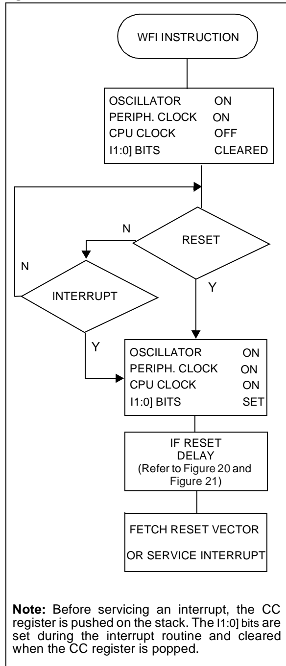
Figure 33. WAIT Mode Flow Chart
