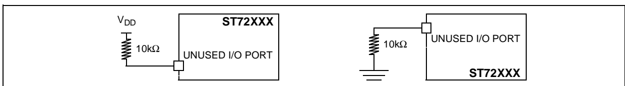
Figure 87 Two typical Applications with unused I/O Pin
