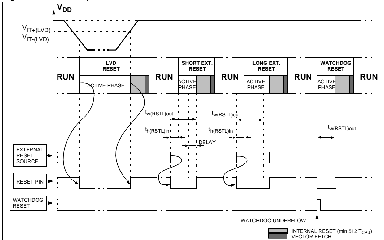
Figure 18. RESET Sequences
