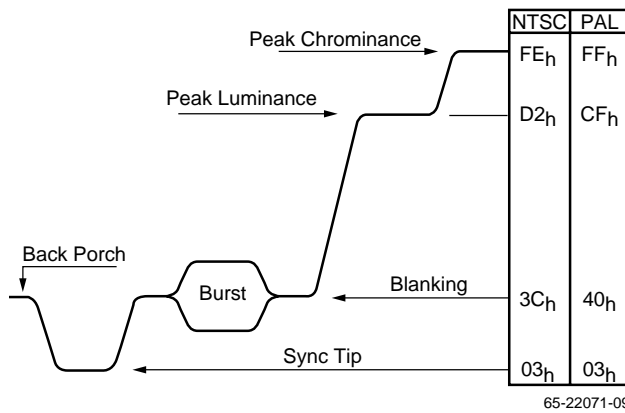
Figure 7. Output Data vs. Input Video Level
