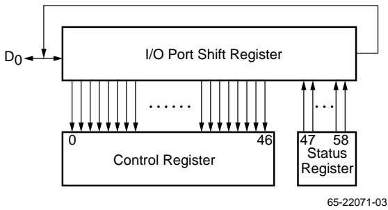
Figure 1. Control and Shift Register Structure
