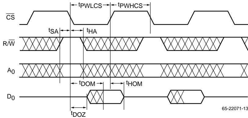
Figure 11. Microprocessor Port – Read Timing
