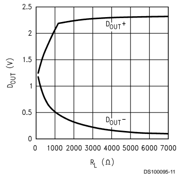
FIGURE 9. Typical DS90LV031A, D_{OUT} vs R_L , V_{CC} = 3.3V , T_A = 25^\circ C
