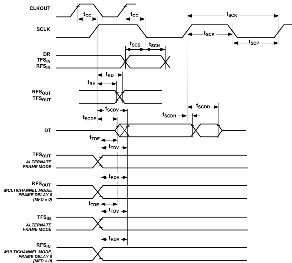
Figure 13. Serial Ports
