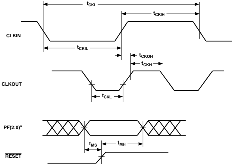
Figure 8. Clock Signals
