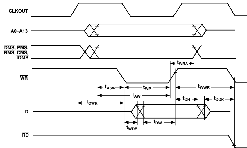
Figure 12. Memory Write
