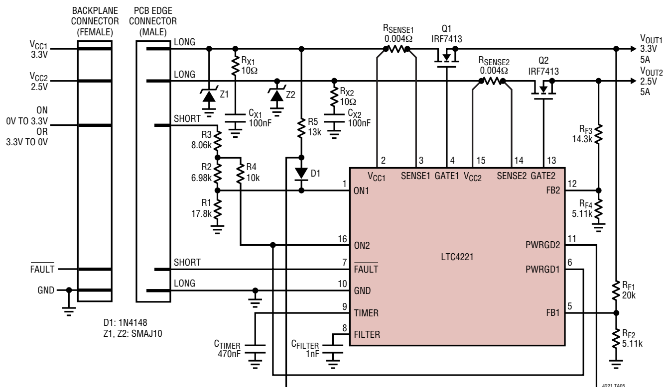
Sequenced Up/Down, Channel 1 Up First, Down Last
