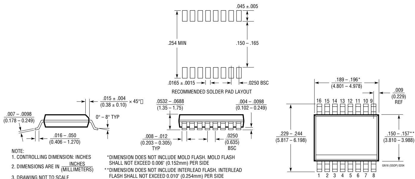
GN Package 16-Lead Plastic SSOP (Narrow .150 Inch) (Reference LTC DWG # 05-08-1641)
