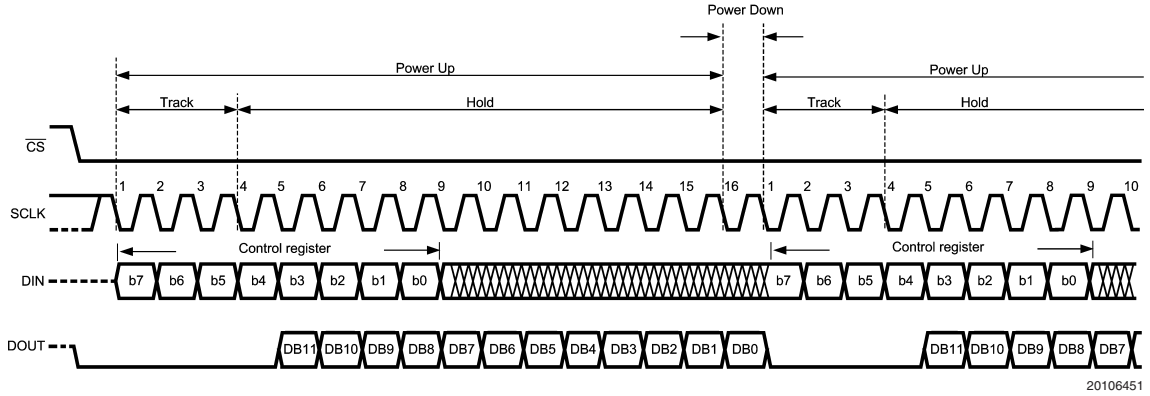
ADC122S051 Operational Timing Diagram
