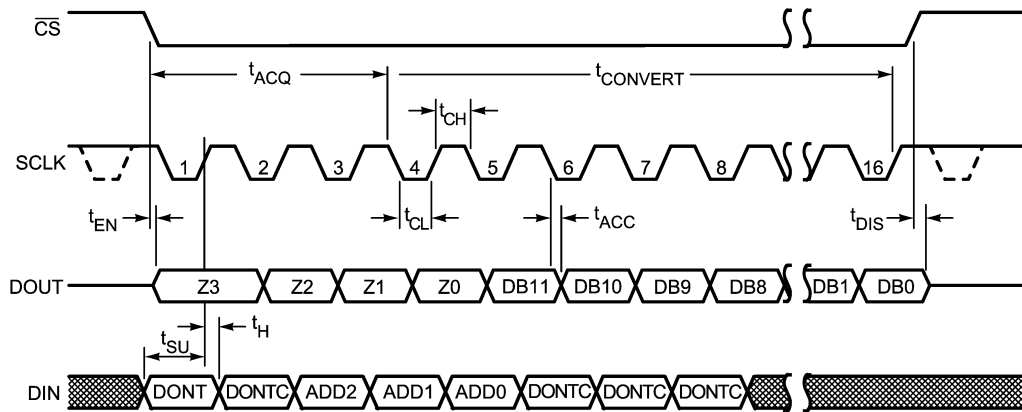
ADC122S051 Serial Timing Diagram
