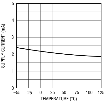
Supply Current in Driver Disable
