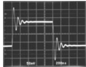
Small-Signal Transient ( A_V = -1, C_L = 500\text{pF} )
