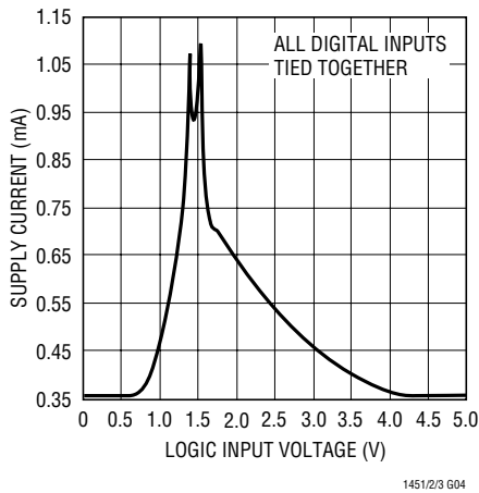
LTC1451 Supply Current vs Logic Input Voltage
