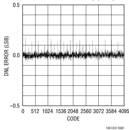
LTC1451 Differential Nonlinearity (DNL)
