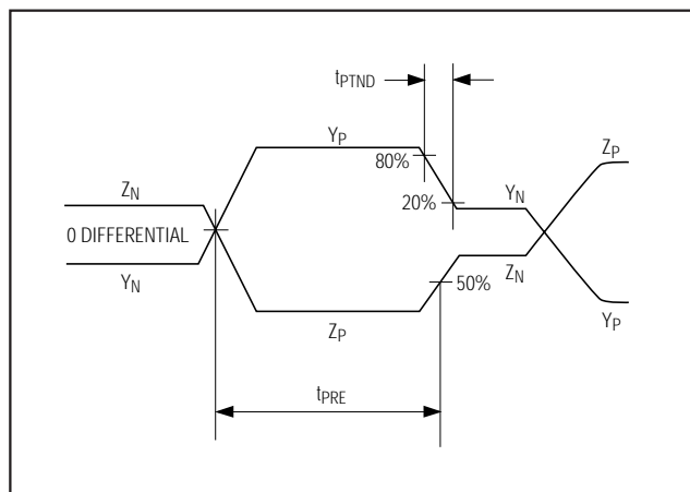
Figure 10. Preemphasis Timing
