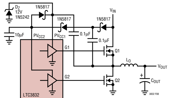
Figure 8. Tripling Charge Pump
