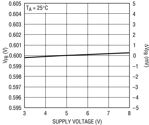
Line Regulation
