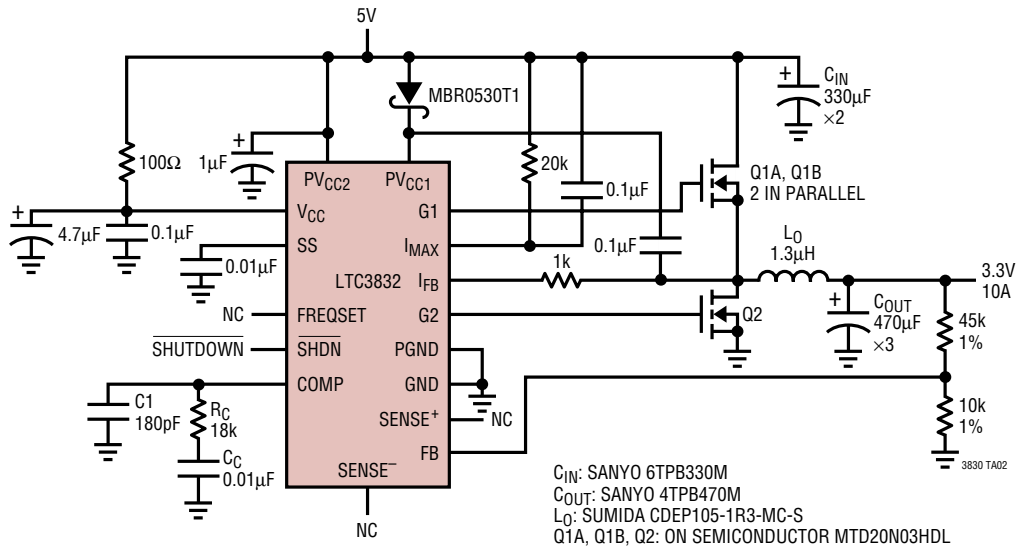
Typical 5V to 3.3V, 10A Application
