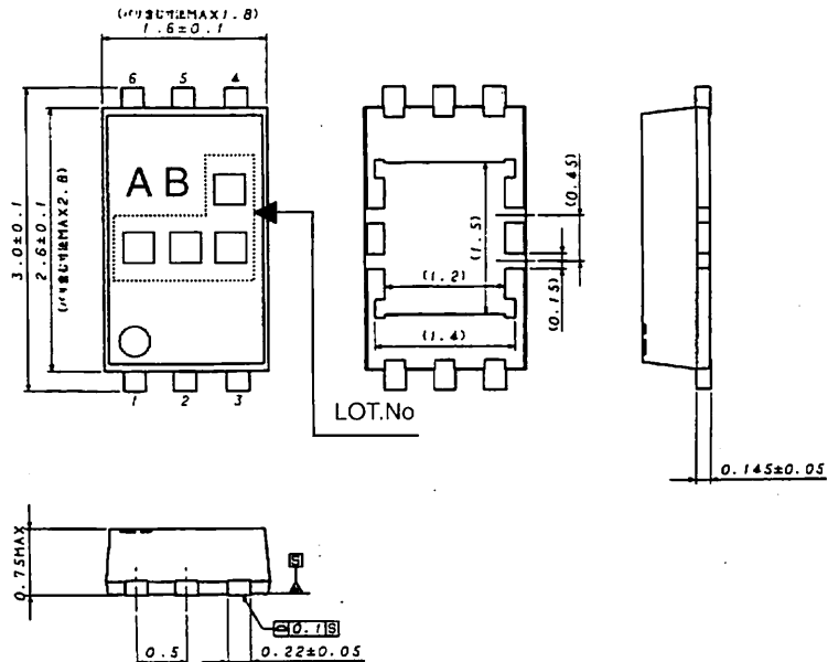
HVSO6-6 (Unit:mm)
