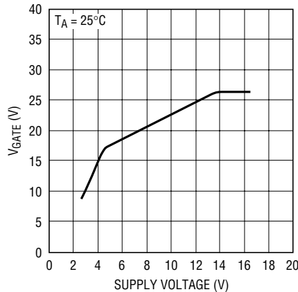
V_{\text{GATE}} vs Supply Voltage
