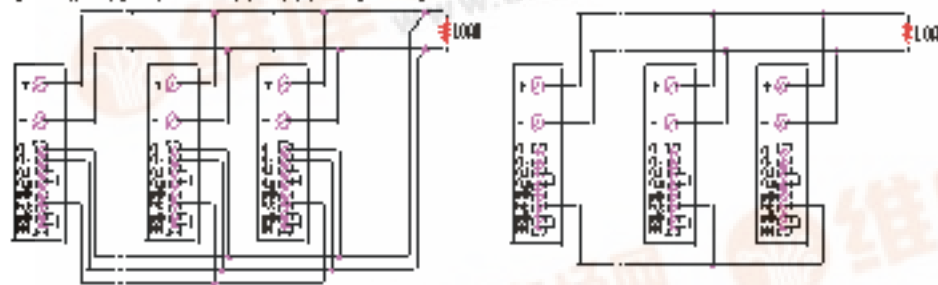
PARALLEL OPERATION WITH REMOTE SENSING
