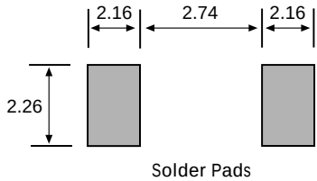
Solder Pads
