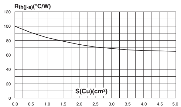
Figure 14: Thermal resistance junction to ambient versus copper surface under each lead (Epoxy printed circuit board FR4, copper thickness: 35 \mu m) (SMB)
