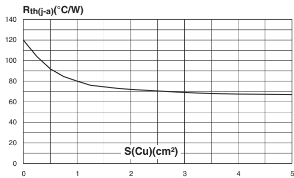
Figure 13: Thermal resistance junction to ambient versus copper surface under each lead (Epoxy printed circuit board FR4, copper thickness: 35 \mu m) (SMA)
