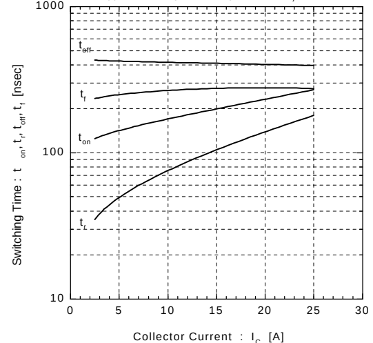
Switching Time vs. Collector Current V_{CC} = 300V, R_G = 16\Omega, V_{GE} = \pm 15V, T_J = 125^\circ\text{C}
