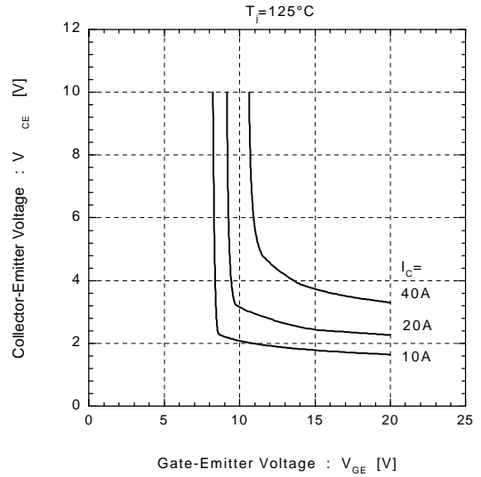
Collector-Emmitter Voltage vs. Gate-Emmitter Voltage
