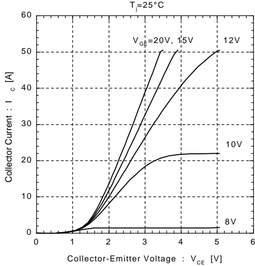
Collector Current vs. Collector-Emmitter Voltage
