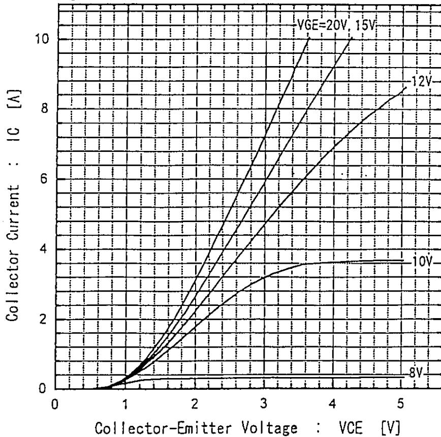
Collector Current vs. Collector-Emmitter Voltage T_j=125^\circ\text{C}
