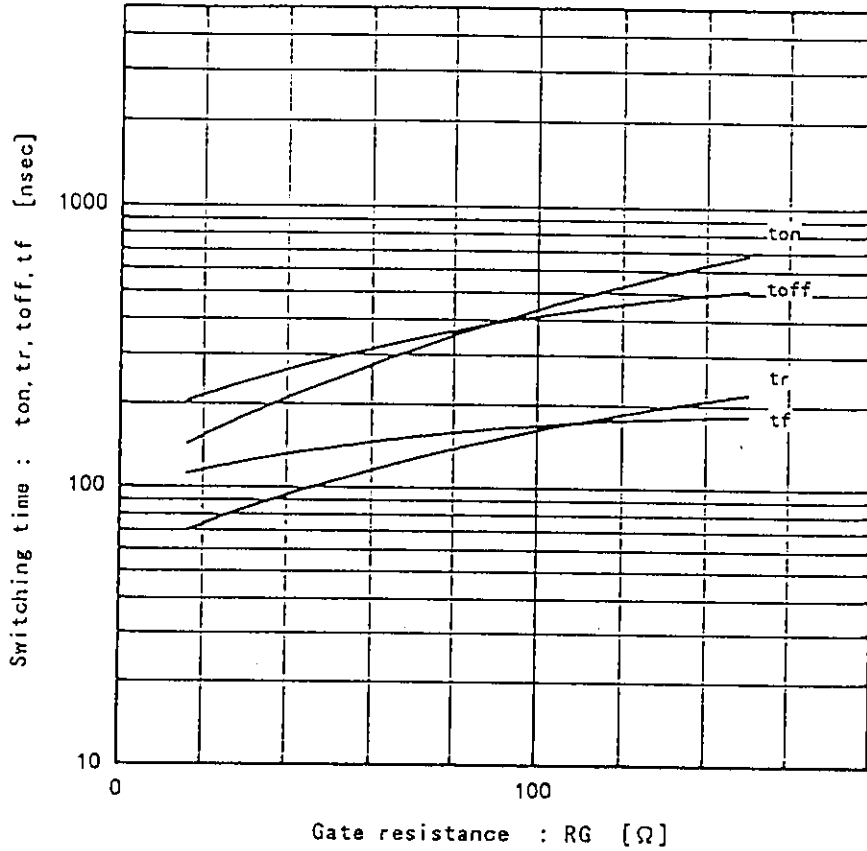
Switching time vs. RG V_{cc}=300V, I_C=15A, V_{GE}=\pm 15V, T_j=25^\circ C
