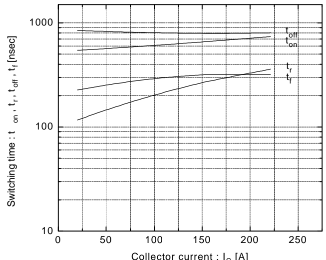
Switching time vs. Collector current V_{CC}=300\text{V}, R_G=16\Omega, V_{GE}=\pm 15\text{V}, T_j=125^\circ\text{C}
