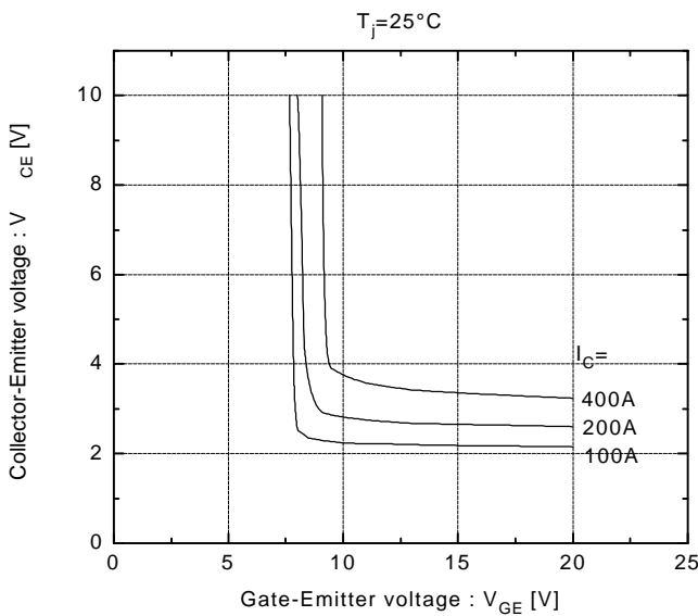
Collector-Emitter vs. Gate-Emitter voltage
