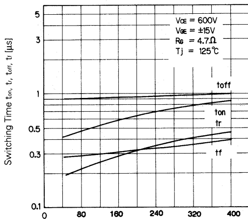
Switching Time
