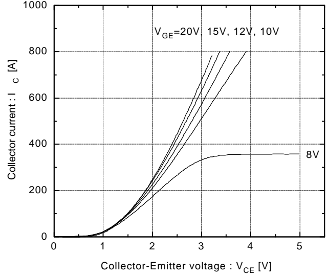
Collector current vs. Collector-Emittter voltage T_j=125^\circ\text{C}
