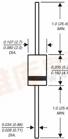
DO-204AL
