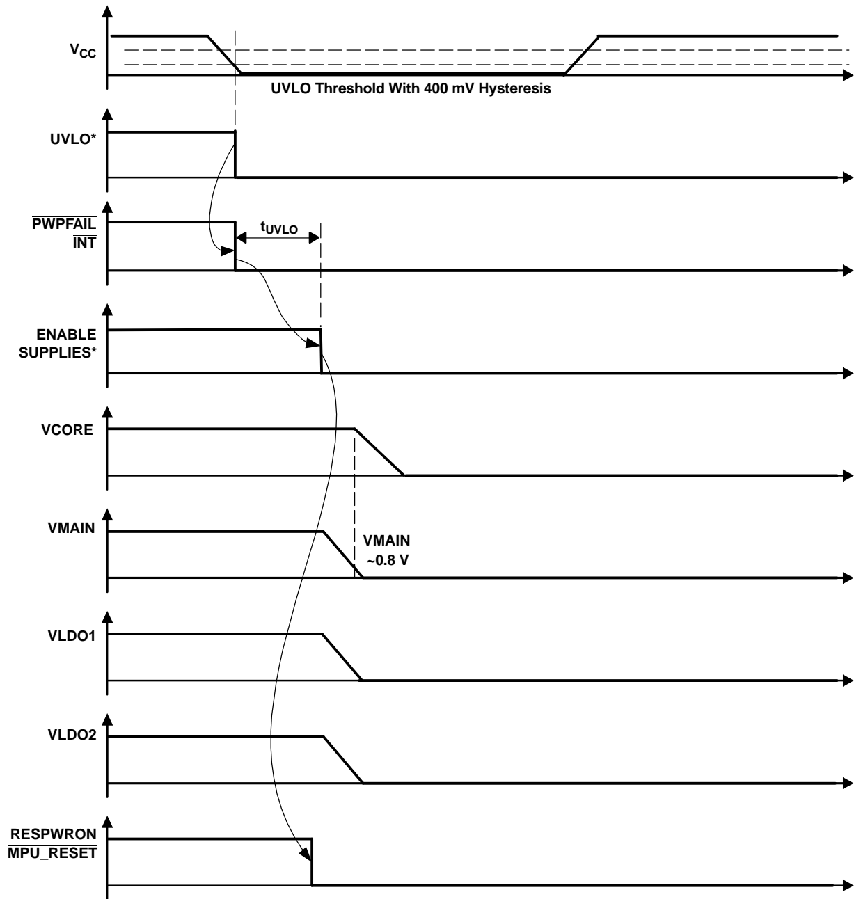
Figure 34. State2-State4 Transition
