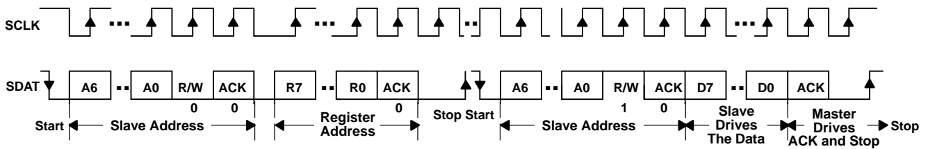
Figure 43. Serial Interface READ From TPS65011: Protocol B
