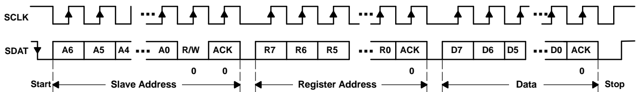
Figure 41. Serial Interface WRITE to TPS65011 Device
