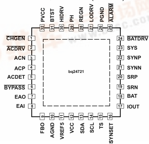
5x5 QFN PACKAGE (TOP VIEW)
