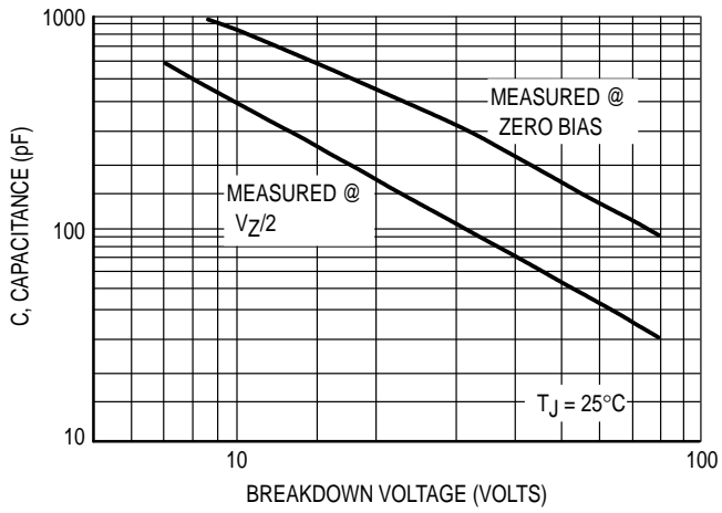
Figure 6. Capacitance Curve
