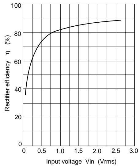
Fig.4 Rectifier efficiency Vs. Input voltage
