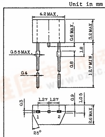
Unit in mm 1. ANODE 2. CATHODE
