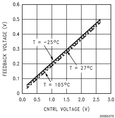
FB Voltage vs. CNTRL Voltage
