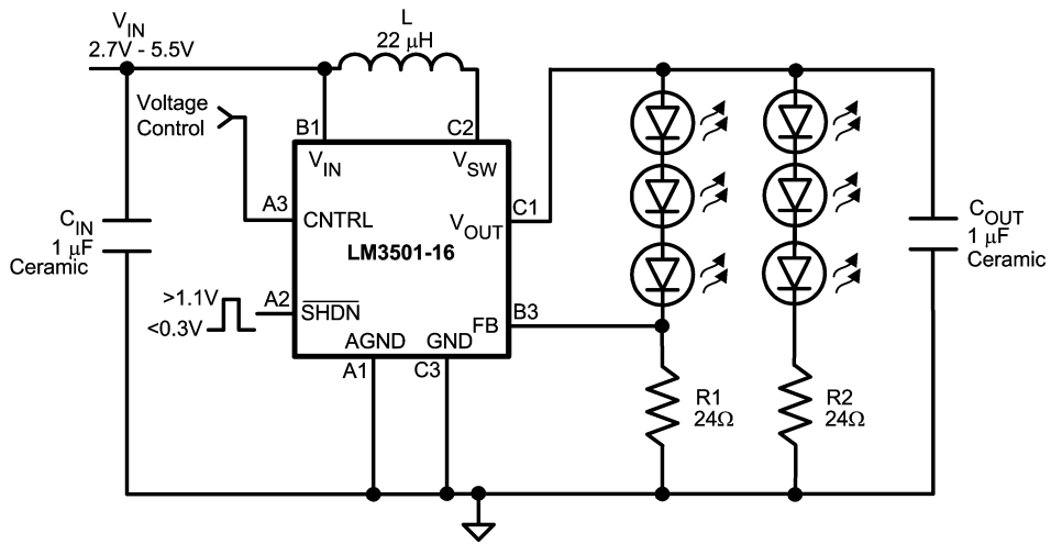
FIGURE 7. Multiple 3 LED String Application
