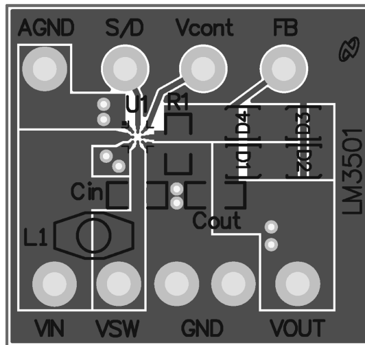
FIGURE 3. Evaluation Board Layout (2X Magnification) Top Layer
