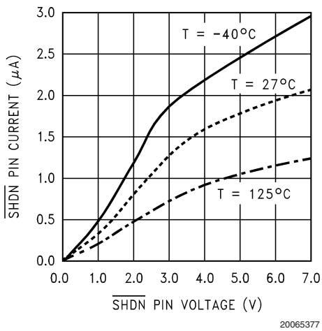
SHDN Pin Current vs. SHDN Pin Voltage
