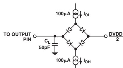
Figure 3. Load Circuit for Digital Output Timing Specification
