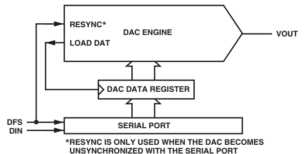
Figure 12. DAC Engine
