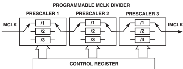
Figure 10. MCLK Divider
