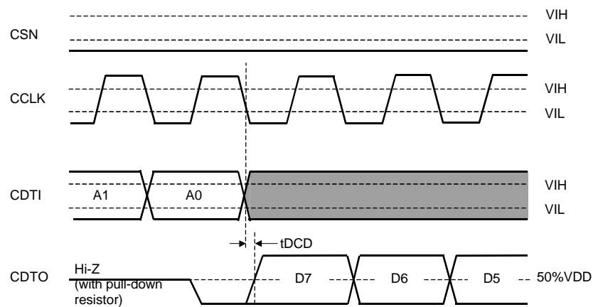
READ Data Output Timing 1
