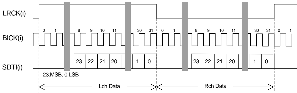
Figure 11. Mode 3 Timing
