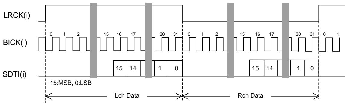
Figure 8. Mode 0 Timing
