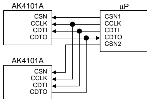
Figure 20. Typical connection with μP Note: External pull-up resistor should not be attached to CDTO pins since CDTO pin is internally connected to the pull-down resistor.
