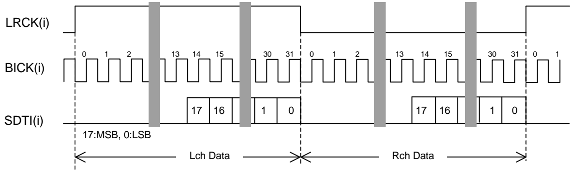
Figure 9. Mode 1 Timing
