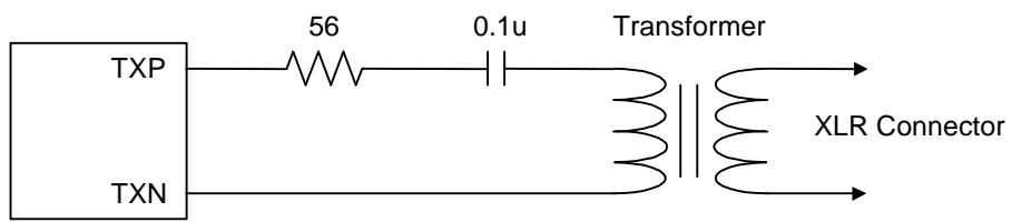
Figure 17. Professional Output Driver Circuit
