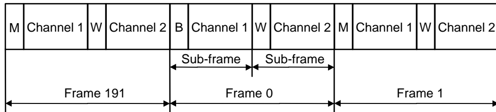
Figure 14. Block format
