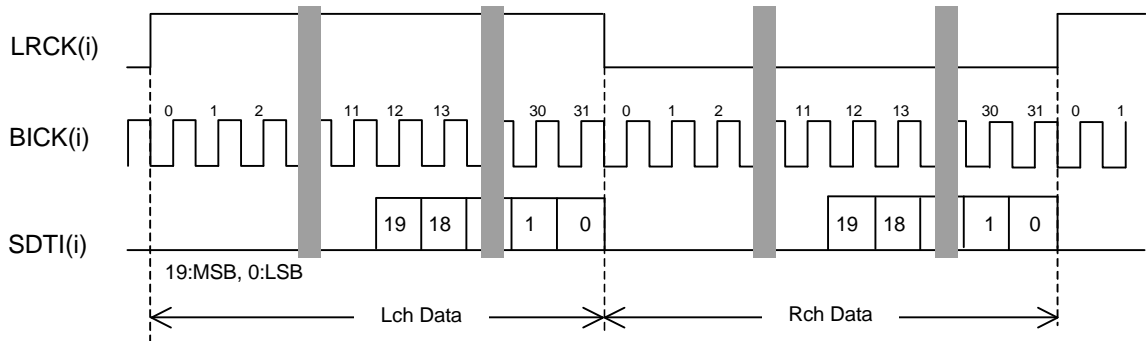
Figure 10. Mode 2 Timing
