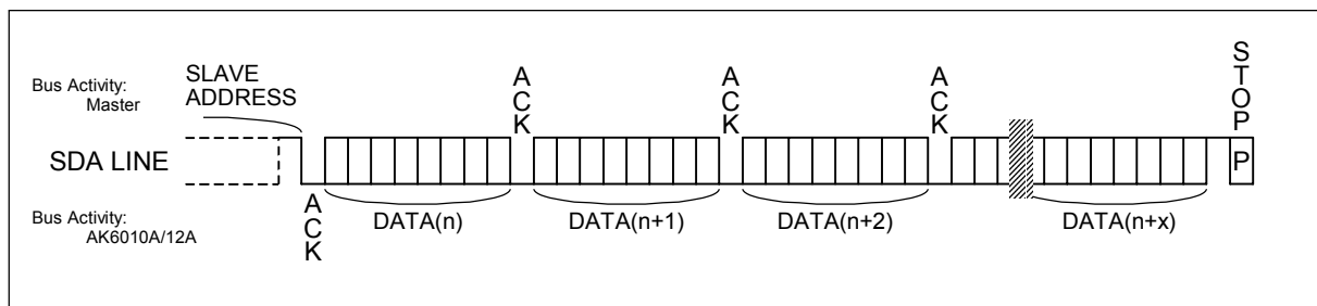
SEQUENTIAL READ
