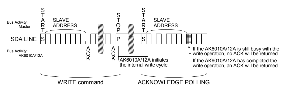
ACKNOWLEDGE POLLING
