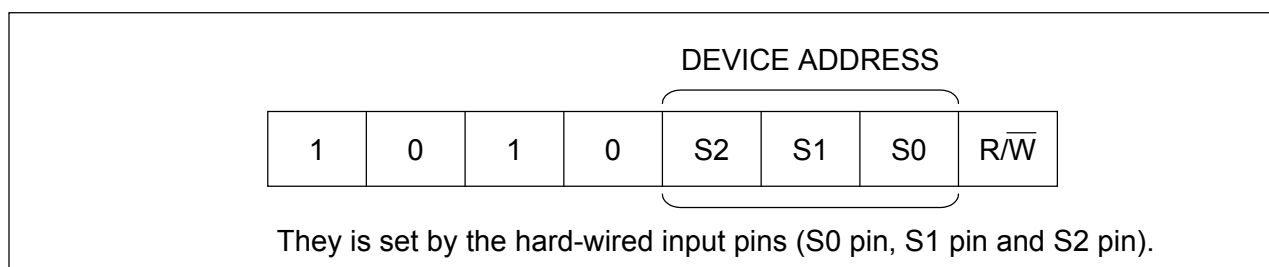
Figure 4. Slave Address
