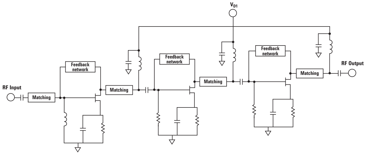
Figure 18. AMMC-5620 Schematic
