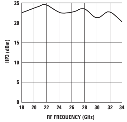
Figure 12. Input 3rd Order Intercept Point, Down Conversion. V_d = 4.5 V, I_d = 150 mA, LO freq = RF - IF.
