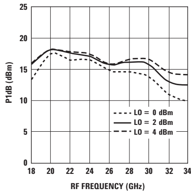
Figure 10. Input Power at 1 dB Conversion Loss, Up Conversion. V_d = 4.5 V, I_d = 150 mA, LO freq = RF + IF.
