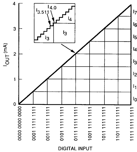
Figure 2. Transfer Characteristic of Segmented Design
