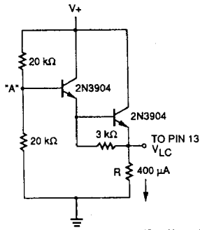
Figure 4. Interfacing Circuits for ECL, CMOS, HTL Logic Inputs
