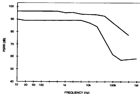
Figure 6. PSRR vs. Frequency
