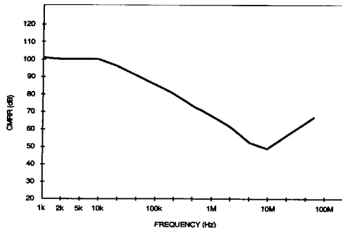
Figure 5. CMRR vs. Frequency
