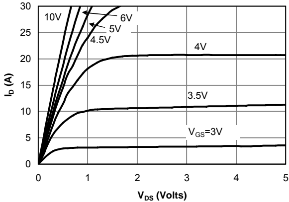
Fig 1: On-Region Characteristics
