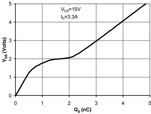
Figure 7: Gate-Charge Characteristics
