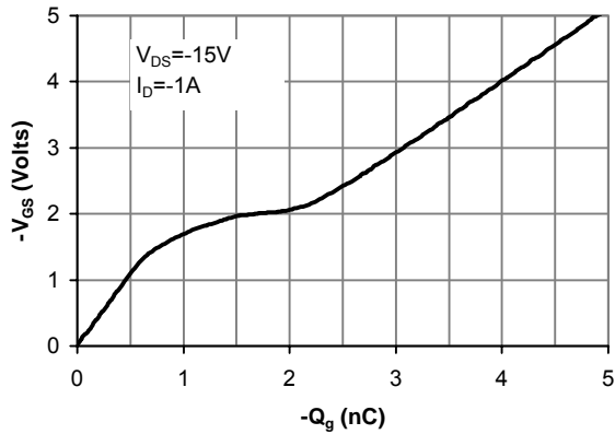
Figure 7: Gate-Charge Characteristics
